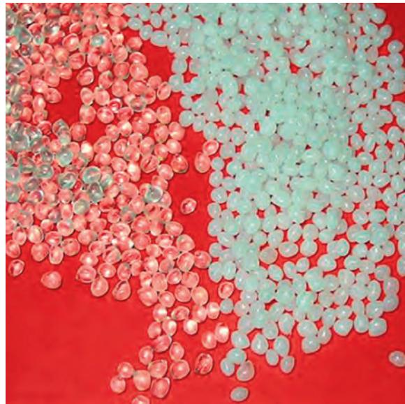
Amorphous pellets (left) compared to Crystalline pellets (right)
